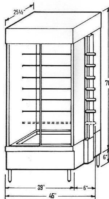
MODEL FL-7 (7 SPITS)
