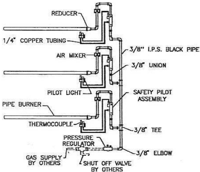
BURNER ASSEMBLY FOR FT-14 GAS MACHINES
