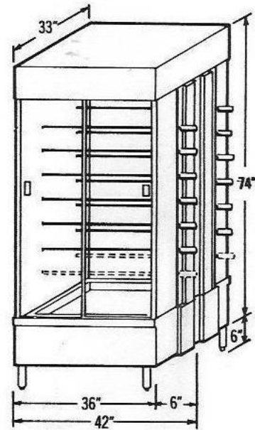
MODEL FT-14 (14 SPITS)
